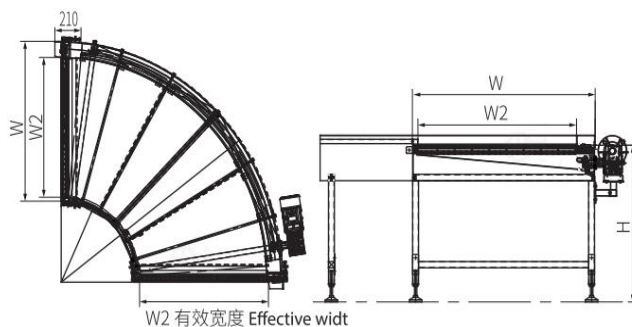
Knife-edge Turning Belt Conveyor
