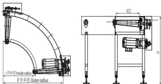
Turning Belt Conveyor
